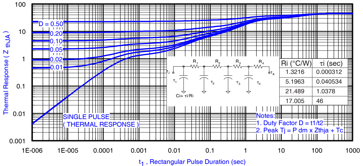
Fig 3. Maximum Effective Transient Thermal Impedance, Junction-to-Ambient ③
